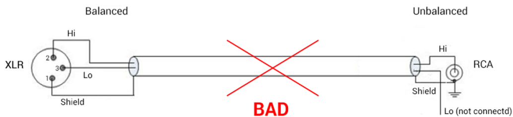
Figure 3 Incorrect balanced output to unbalanced input connection method
