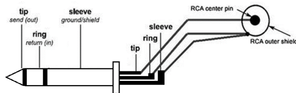
Figure 4 Correct balanced TRS output to unbalanced RCA connection method
