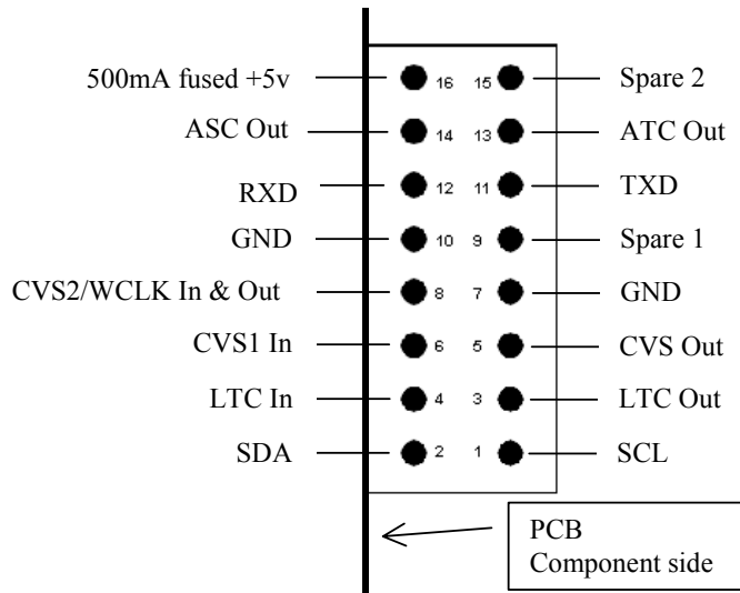
Figure 5 - Video/TC Header Pin-out
