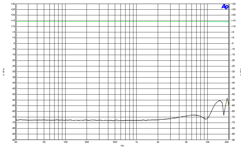
Figure 7 - Monitoring frequency response measurement
