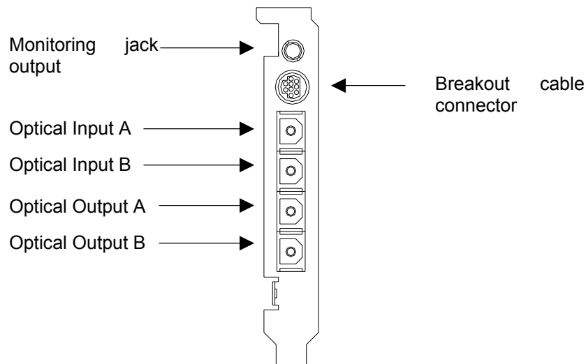
Figure 9 - Mykerinos & ADAT daughter card connectors
