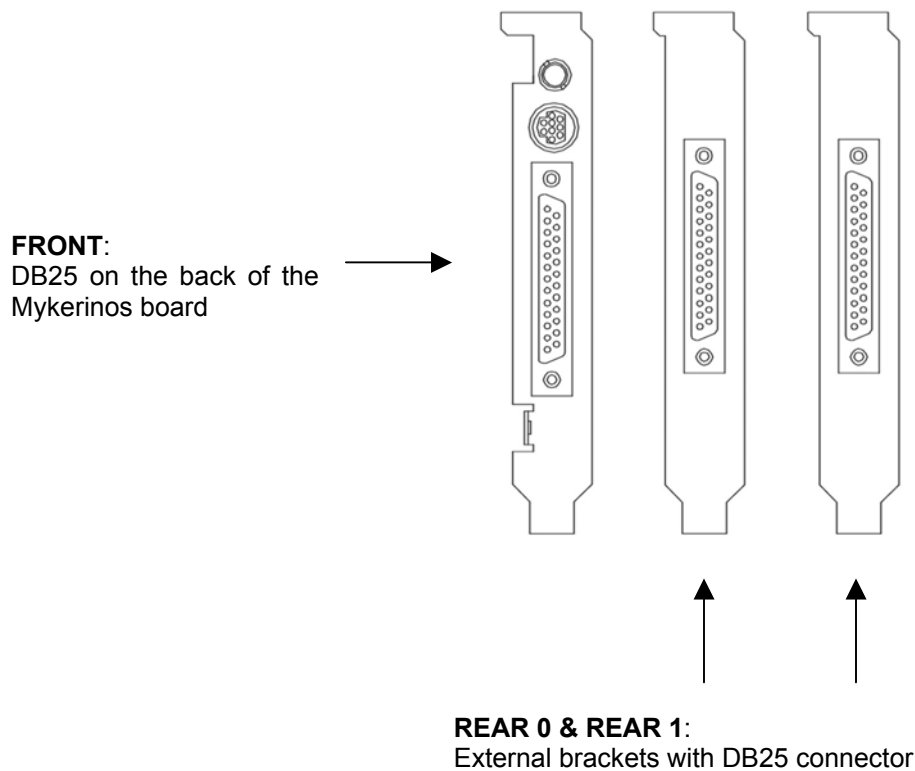
Figure 13 - Mykerinos & AES-EBU/SDIF/TDIF daughter card DB-25 connectors
