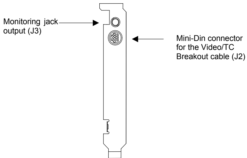
Figure 3 - Mykerinos Bracket with Jack & mini-Din connectors
