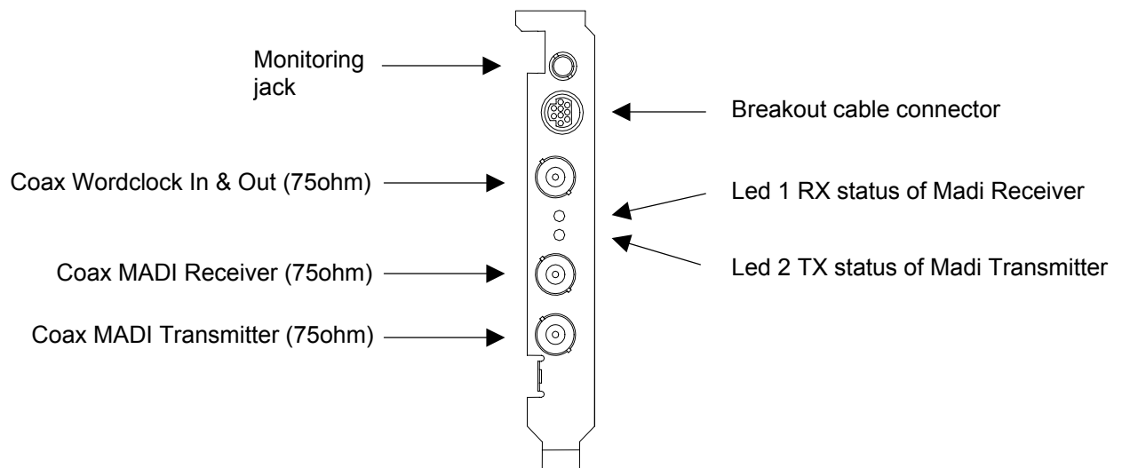
Figure 10 – Mykerinos & coaxial MADI daughter card connectors
