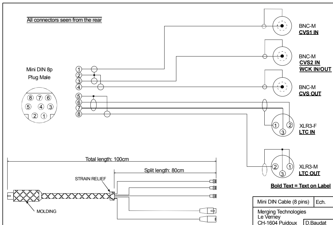
Figure 4 - Breakout Cable Pin-out
